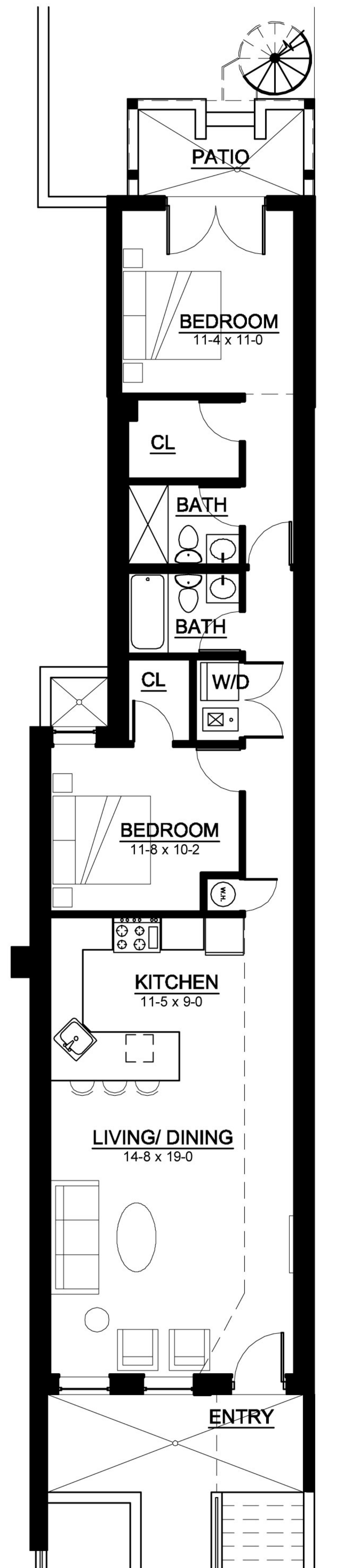
GARDEN LEVEL PLAN
