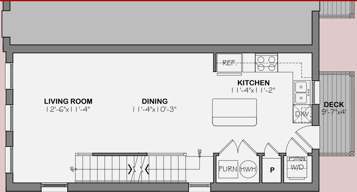
SECOND FLOOR
